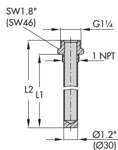
Thermowell for flammable gases 1 NPT/Class 600
