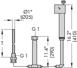
Types 2232/2234 Control Thermostats
