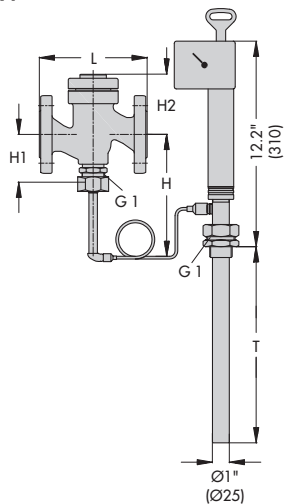
Type 1u Temperature Regulator with Type 2231 or 2233 Control Thermostat
